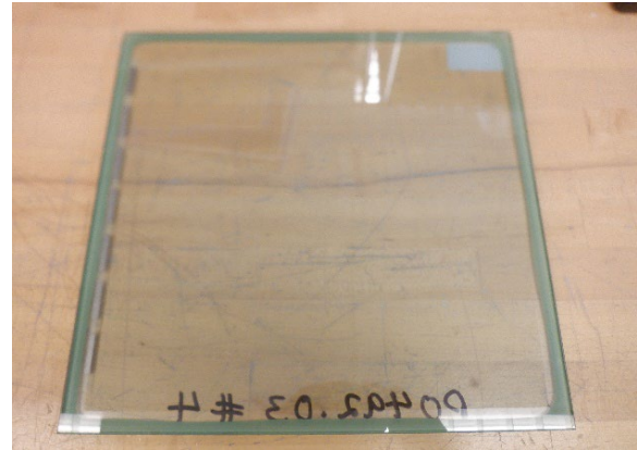
VIG Specimen - 5S1.16+0.15V+5, (Sample 4)
